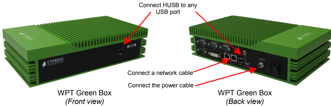
Figure 1. Connections to the WPT Green Box
